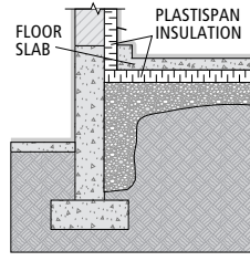
Horizontal Insulation
