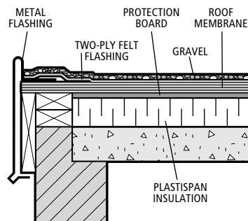
Gravel Stop
