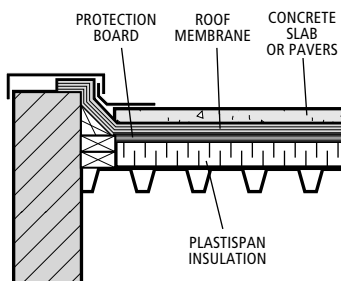
Traffic Deck
