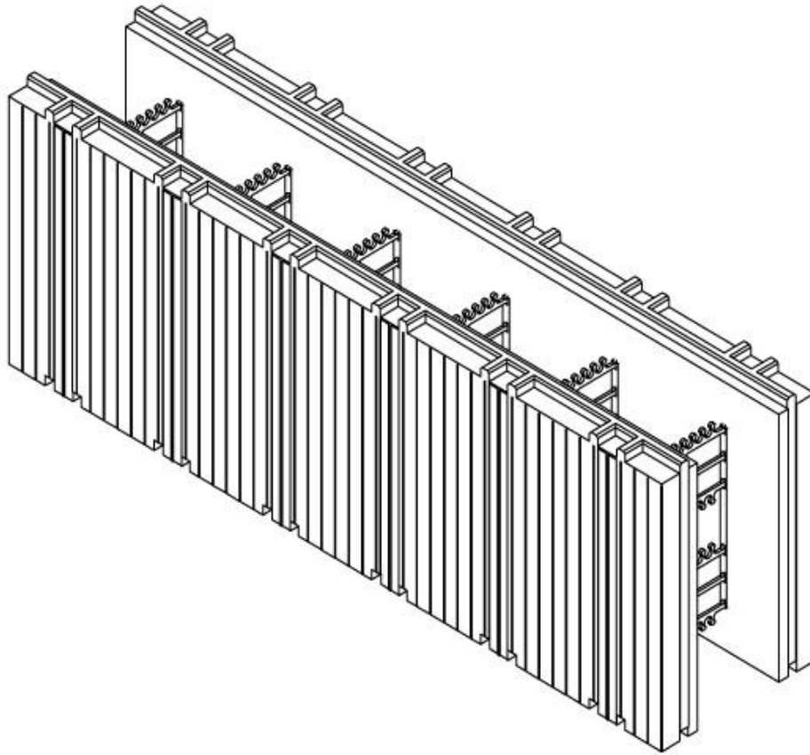
Figure 1. “Advantage Insulating Concrete Forming (ICF) System” standard unit
